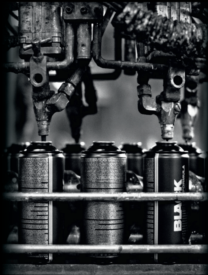
Production of the Montana BLACK series in Haßmersheim Germany, Filling line.
